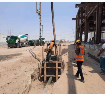
Piling and drilling rig
